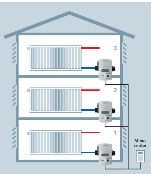
M-bus: data collection via the M-bus center using a two-wire bus
